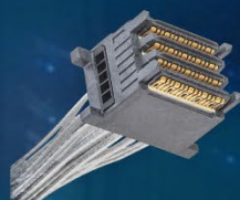
ExaMAX2® cable
